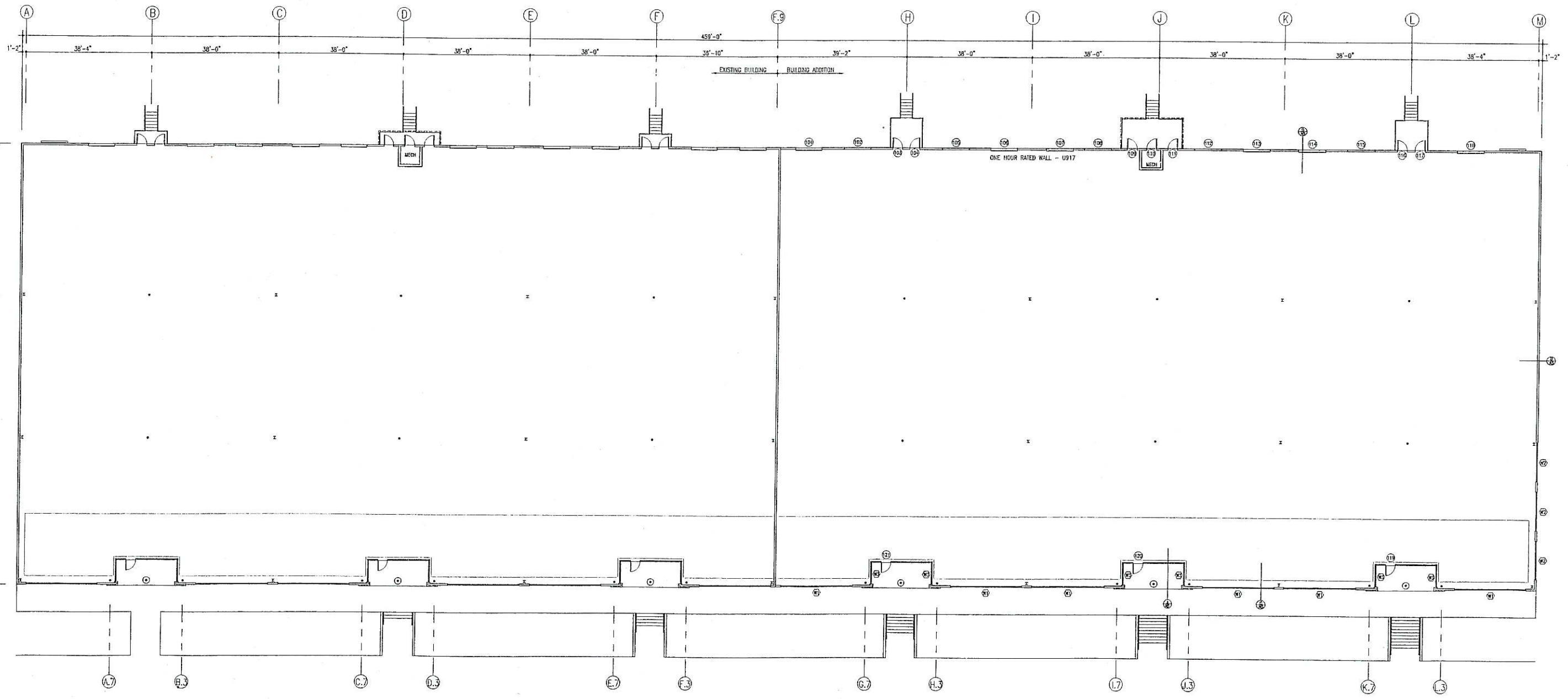
OVERALL FLOOR PLAN SCALE 1/16" = 1'-0"
